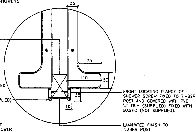
DETAIL B TYPE 750 C - BANKING DETAIL
