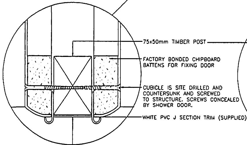
PLAN OF BANKED SHOWERS
