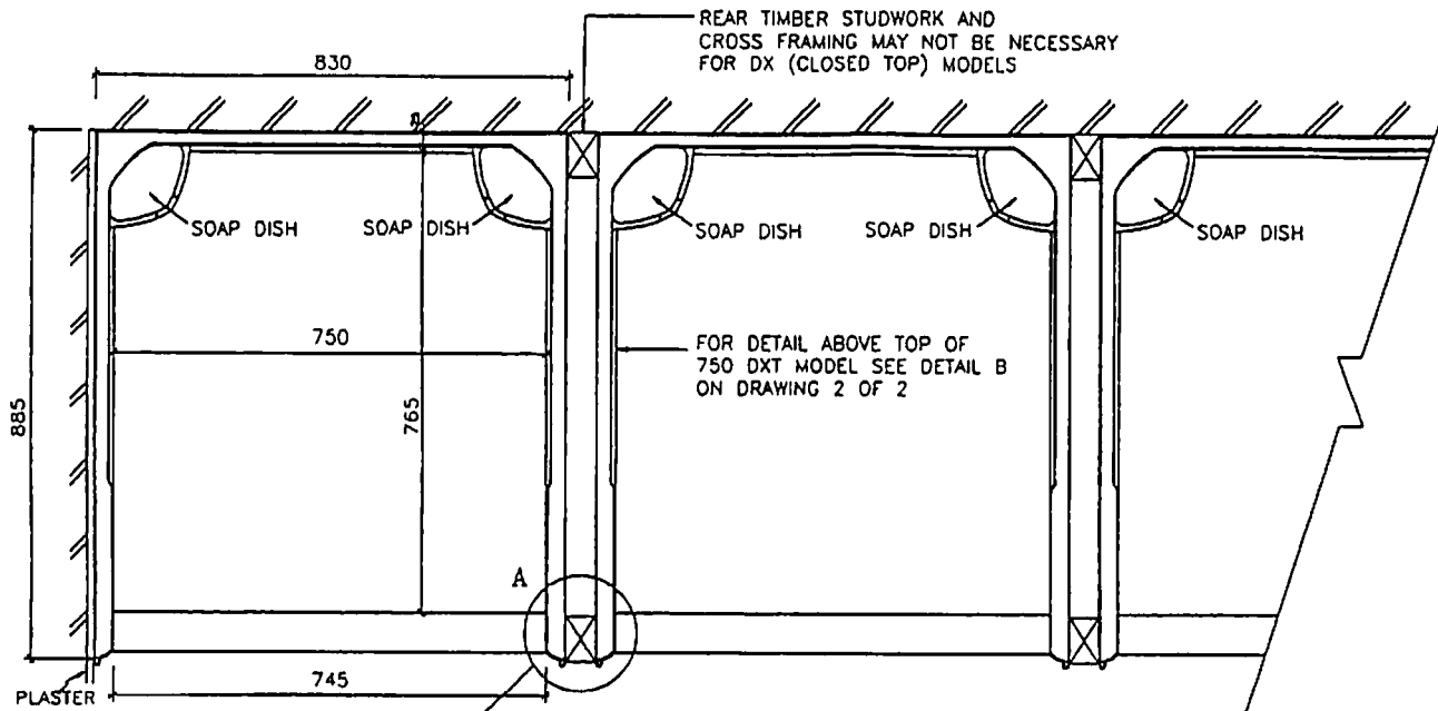
PLAN OF BANKED SHOWERS
